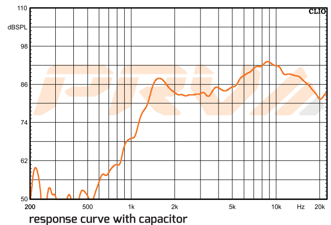
Frequency Response Measured at 2.00V/1m
