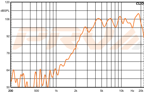
Frequency Response Measured at 2.00V/1m
